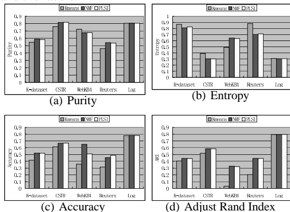
Figure 1: Performance Comparison of NMF and PLSI
