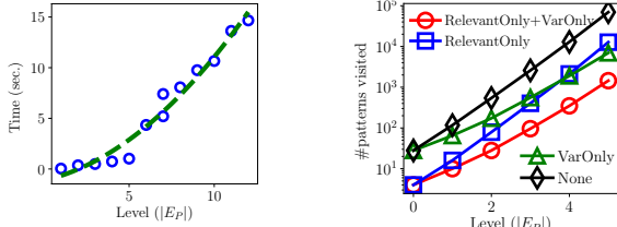
Figure 10: Time spent by Context Evaluator (Alg. 2) on evaluating patterns at different levels.
