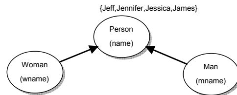
Figure 6: Subtype and value constraints
