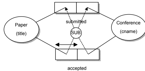
Figure 5: Subset constraint
