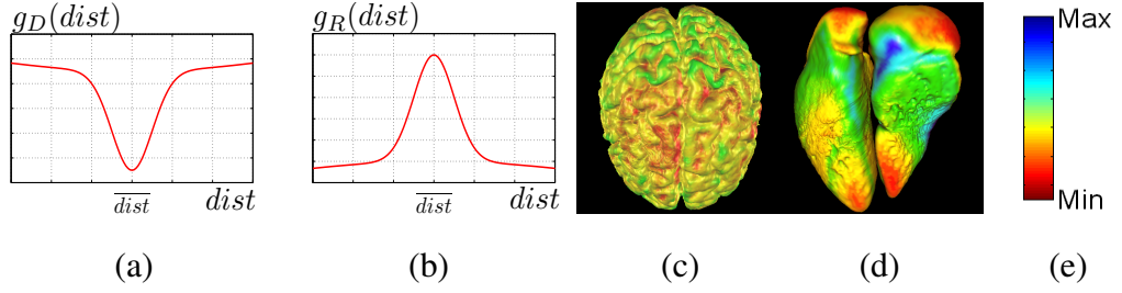
Figure 7: (a)(b) Functions to balance the contributions of region term and spatial constraint term, (c) DC mapping of brain gray matter segmentation; the range for distance between Gray and white matters is 2~15 voxels, (d) DC mapping of heart segmentation; the distance range is 2~25 voxels, (e) the color bar used to map the spatial information.
