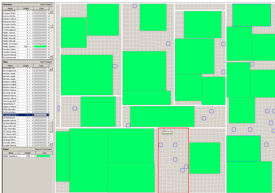
Figure 4: The context can be used to formulate queries. Therefore, all items of the context treemap can be selected and deselected by mouse clicks, and the resulting query is visualized by red borders. Similarly, selecting a fund or set of funds in the overview, filter, or depot view (Prudential is selected in the Filter here) emphasizes the stocks owned by the fund(s) via blue borders.
