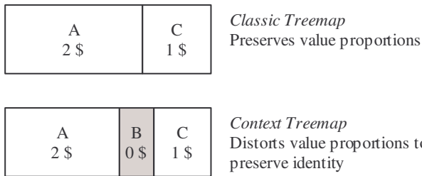
Figure 2: A classic treemap and a Context Treemap displaying the same data set.
