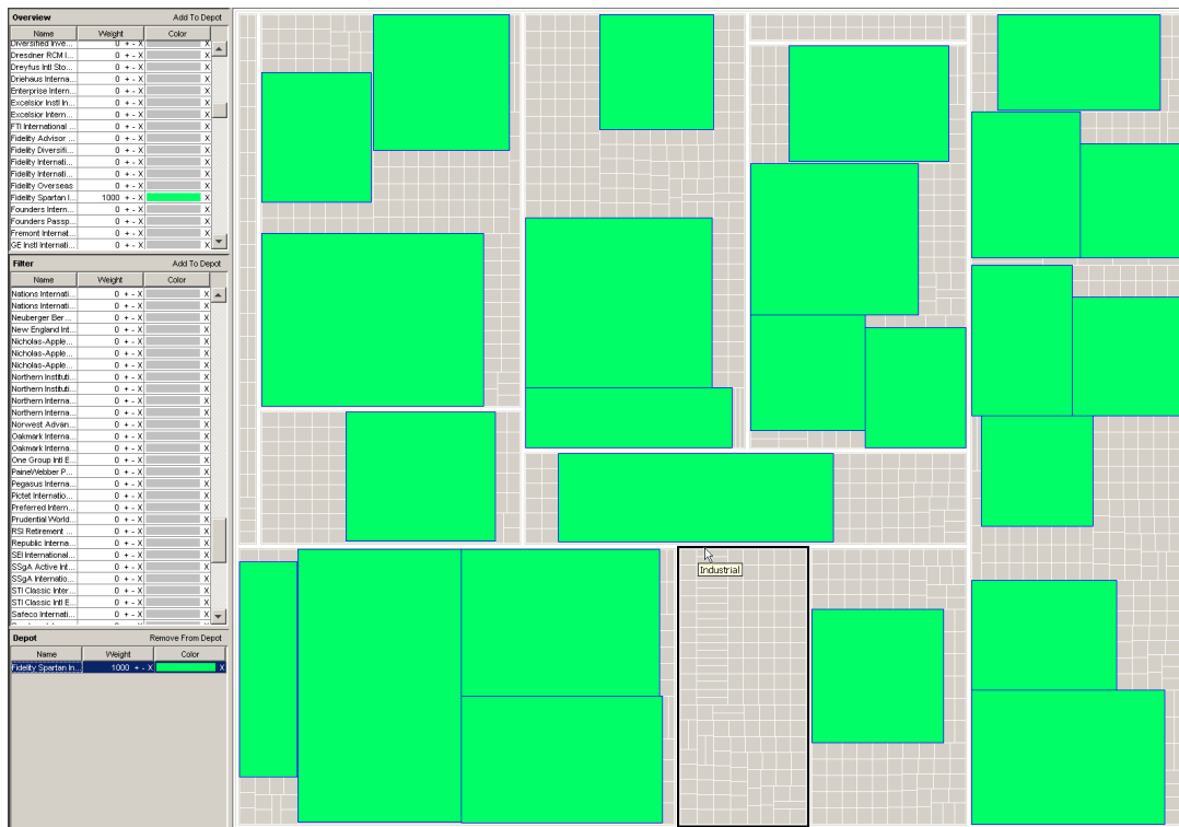
Figure 3: Visualizing one fund with FundExplorer. On the left side, FundExplorer lists from top to bottom: all funds, the funds returned by the current filter and the funds that are part of the depot. On the right side, the context treemap displays the owned fund embedded in its context. Moving the mouse across the context treemap activates tooltips that describe the items pointed at.
