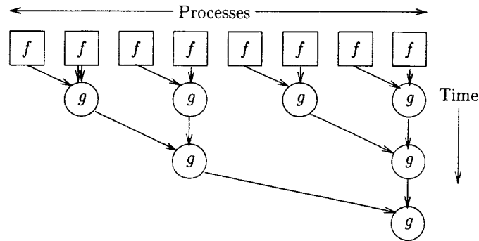
Figure 3. A skeleton for computing arbitrary list homomorphisms.
