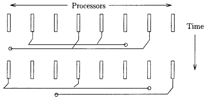
Figure 5. A communication skeleton.
