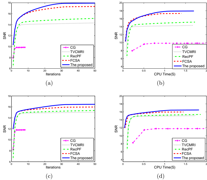
Fig. 3: Performance comparisons on: a)b) The Cardiac image; c)d) The Chest image. All algorithms are without total variation regularization.
