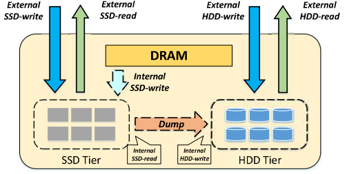
Figure 2: The architecture and IO flows of hybrid WSN comprising an SSD and an HDD Tier.
