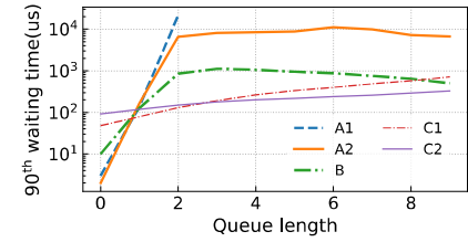
(a) The 90 th -percentile waiting delay.
