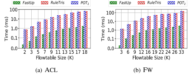
Fig. 2. Compute time comparison on different Flow tables.
