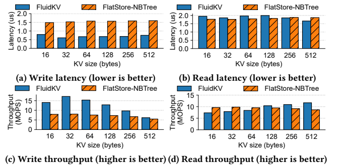
Figure 18: Write/read performance with different KV sizes.
