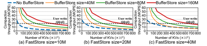
Figure 15: Compaction efficiency with different FastStore and BufferStore configurations.
