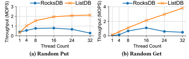
Figure 4: The performance of LSM-tree-based KVS [OB4].
