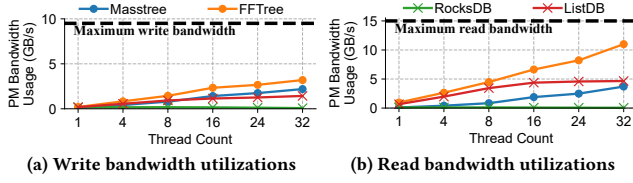
Figure 5: I/O bandwidth utilizations of single- and multi-stage indexing KVSs when loading 200M KV (3 GB) [OB5].
