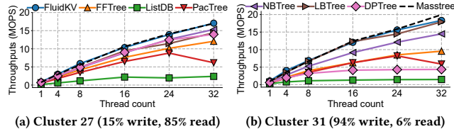
Figure 14: Performance under Twitter cluster workloads.
