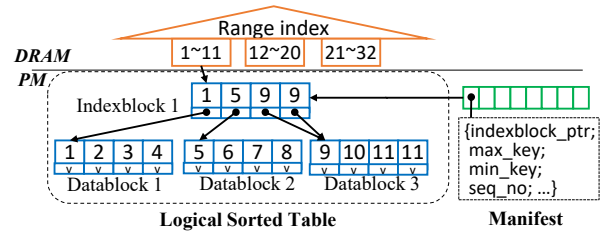
Figure 9: Data structures in StableStore.
