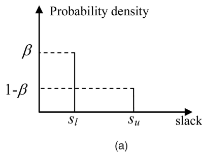
Fig. 2. Slack distribution. (a) Two-spike distribution. (b) Uniform distribution.
