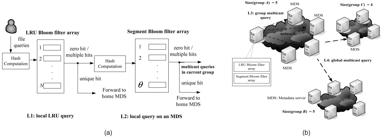
Fig. 1. The group-based HBA architecture allowing the multilevel query. (a) LRU and segment Bloom filter arrays allowing the L1 and L2 queries. (b) L3 and L4 queries, respectively, in a group and entire system.
