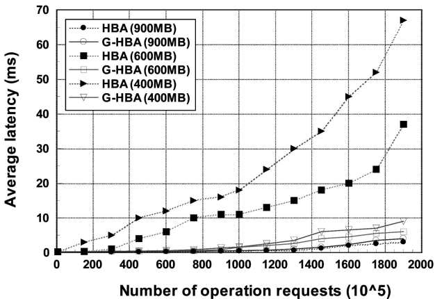
Fig. 5. Average latency comparisons of HBA and G-HBA with different memory sizes under the INS trace.
