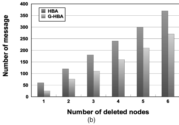
Fig. 13. The message numbers when adding and deleting nodes using HP trace. (a) Inserting nodes. (b) Deleting nodes.
