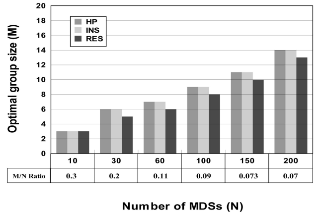
Fig. 3. Optimal group size as a function of the number of nodes.
