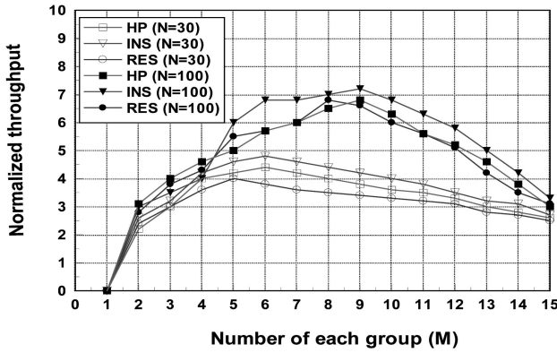
Fig. 2. Normalized throughput of G-HBA when the total number of MDSs is 30 and 100 MDSs, respectively.
