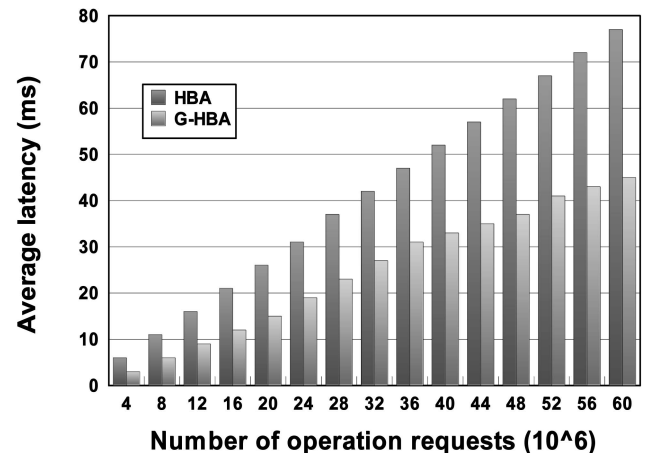
Fig. 12. Average query latency using intensified EECS trace.
