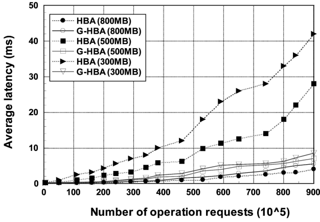
Fig. 4. Average latency comparisons of HBA and G-HBA with different memory sizes under the RES trace.
