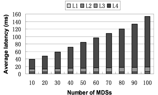
Fig. 10. Query latency in different levels.
