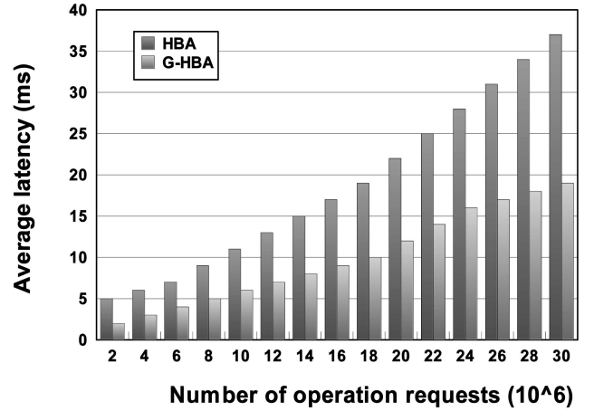
Fig. 11. Average query latency using intensified HP trace.
