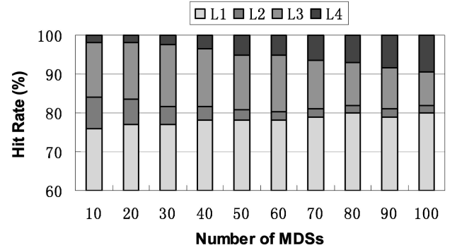
Fig. 9. Percentage of queries successfully served by different levels.
