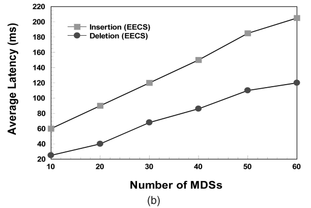
Fig. 14. Average latency when adding and deleting one node using HP and EECS traces. (a) HP trace. (b) EECS trace.
