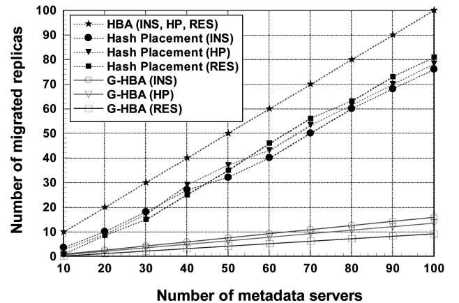
Fig. 7. Number of migrated replicas using HBA, hash-based placement, and G-HBA schemes.
