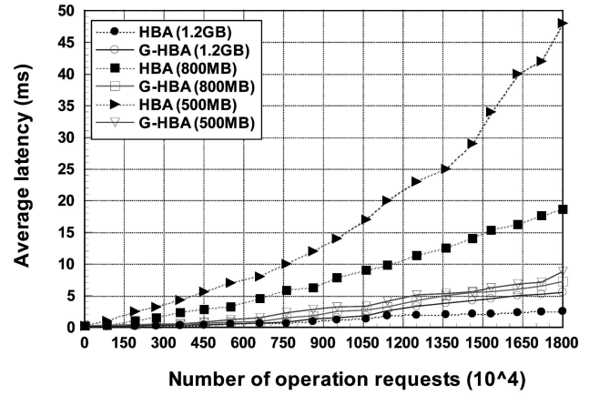
Fig. 6. Average latency comparisons of HBA and G-HBA with different memory sizes under the HP trace.
