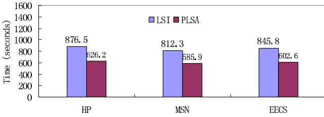
Fig. 6. Initial construction time by using LSI and PLSA.
