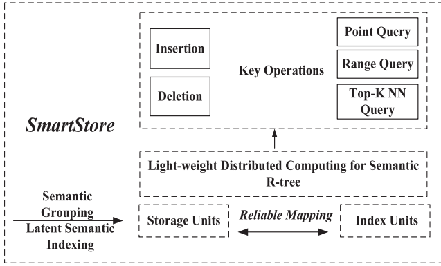
Fig. 2. SmartStore system diagram.
