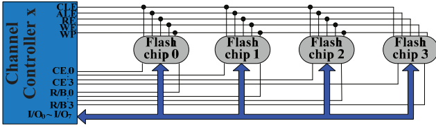
Fig. 2. The connection of an independent channel.
