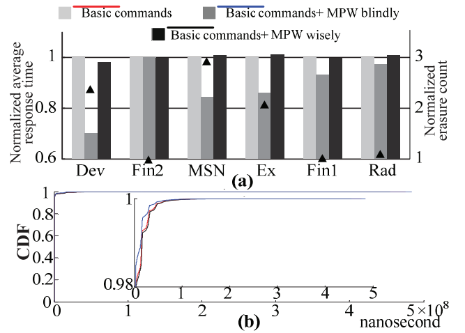
Fig. 10. (a) Performance and endurance impacts of the two methods of using the MPW command; (b) CDF of the response time.
