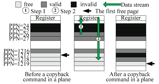
Fig. 7. An example of the copyback command.
