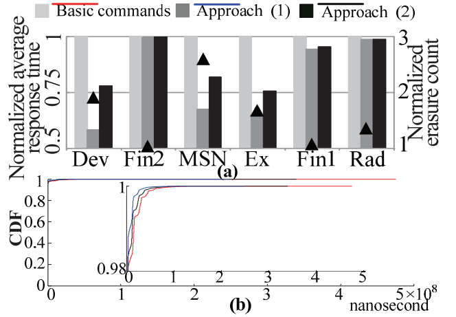
Fig. 13. (a) Performance and endurance impacts of the two recommended approaches to the combined use of the advanced commands; (b) CDF of the response time.
