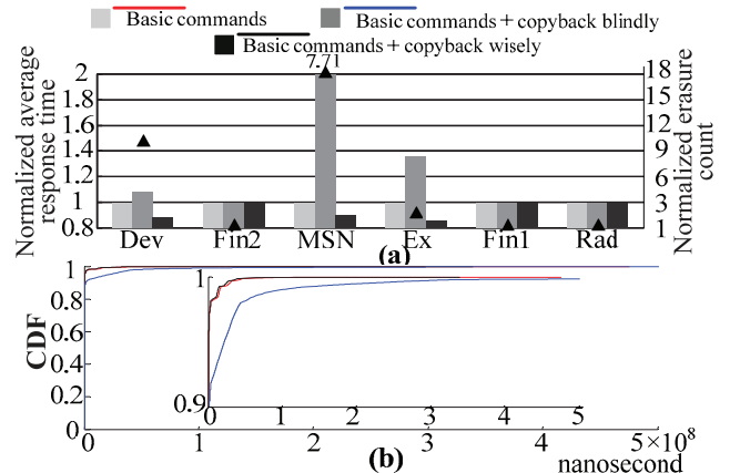
Fig. 8. (a) Performance and endurance impacts of the two methods of using copyback command; (b) CDF of the response time.
