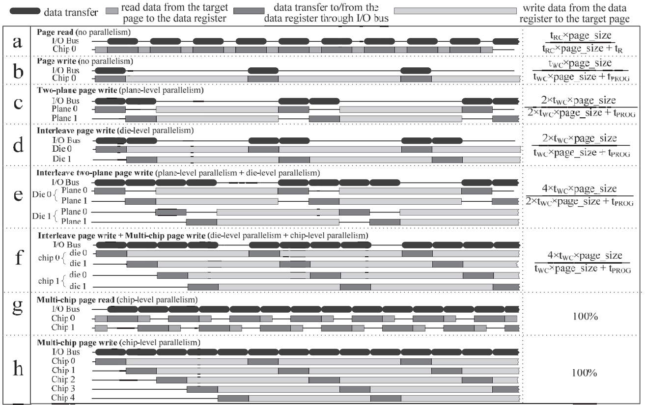
Fig. 19. The utilizations of exploiting different levels of parallelism.
