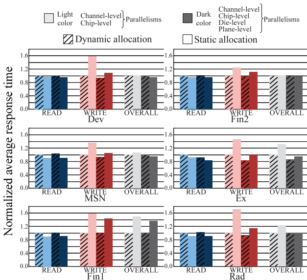
Fig. 15. Performance impact of different allocation schemes, measured in the average response time normalized to that of dynamic allocation with only the channel-level and chip-level parallelism.
