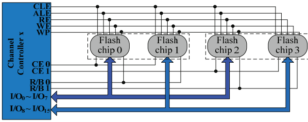
Fig. 20. The bit extension channel.
