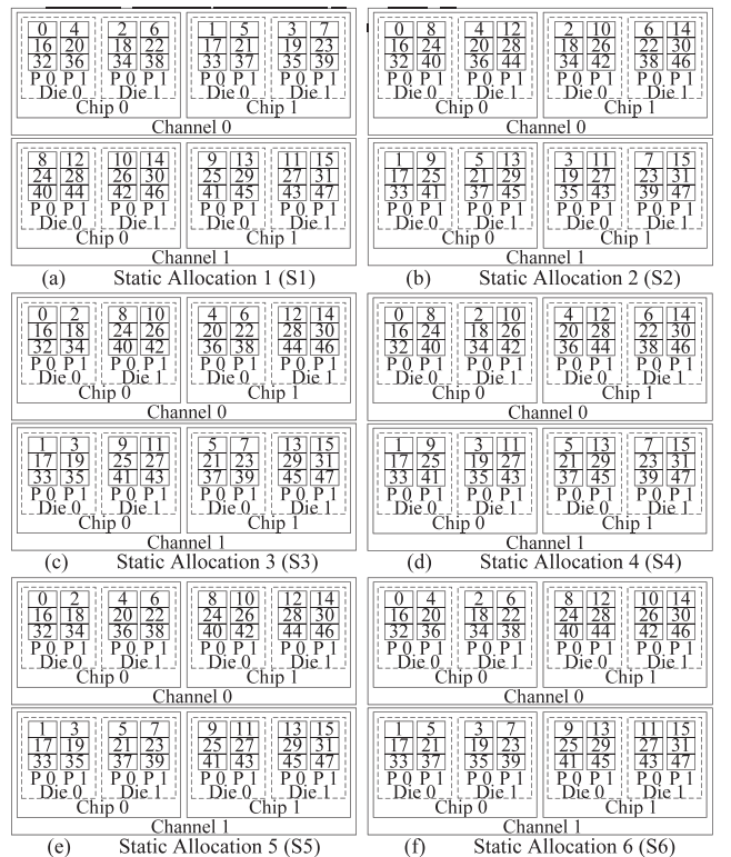
Fig. 14. The six typical static allocation schemes.
