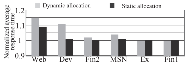
Fig. 11. Performance gain of MPR over the basic commands under the dynamic and static allocation schemes, respectively.
