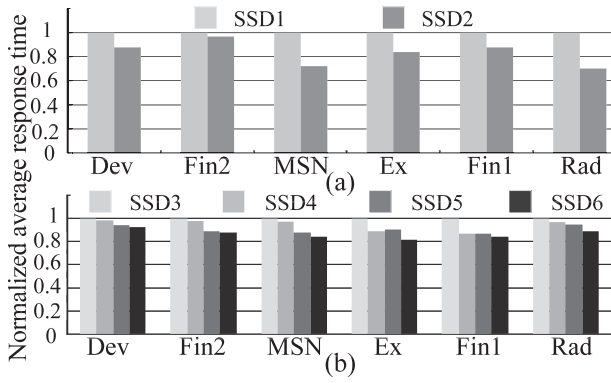
Fig. 17. Normalized average response time of SSD1, SSD2, SSD3, SSD4, SSD5, and SSD6.
