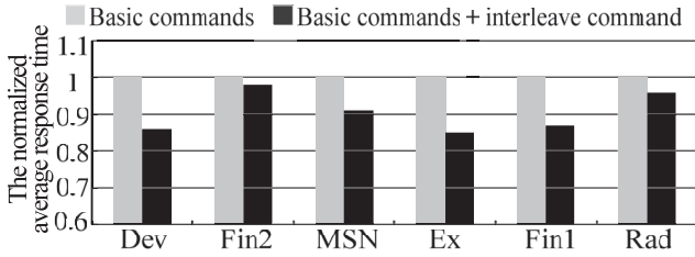
Fig. 12. Performance impact of the interleave command.
