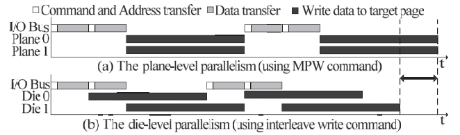
Fig. 16. The plane-level parallelism versus the die-level parallelism.
