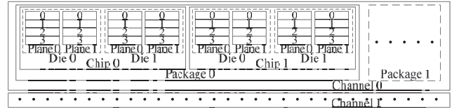
Fig. 3. An SSD internals.
