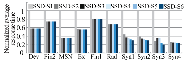
Fig. 18. Normalized average response time of SSD-S1, SSD-S2, SSD-S3, SSD-S4, SSD-S5, and SSD-S6.
