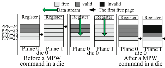
Fig. 9. An example of using the MPW command.
