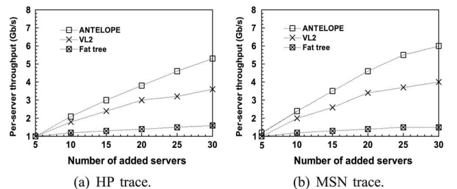
Fig. 14. Per-server throughput.
