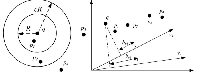
Fig. 6. An example of LSH working scheme.
