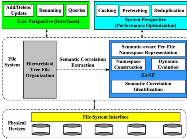
Fig. 2. SANE as a middleware in file systems.
