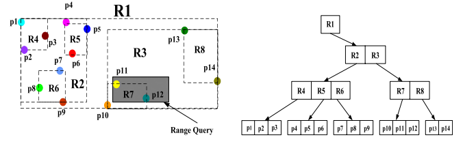
(a) The data representation in geometric space.
