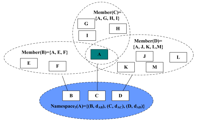
Fig. 4. Two-set representation for speedy update.
