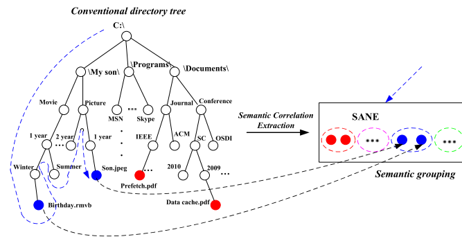
Fig. 1. SANE and hierarchical directory tree.
