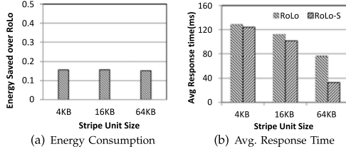
Fig. 10. Energy consumption and performance comparison between RoLo and RoLo-S as a function of the stripe unit size under src2.2 .
