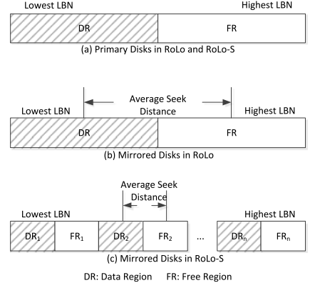
Fig. 5. Data regions and free regions distribution of primary disks and mirrored disks in both RoLo and RoLo-S.
