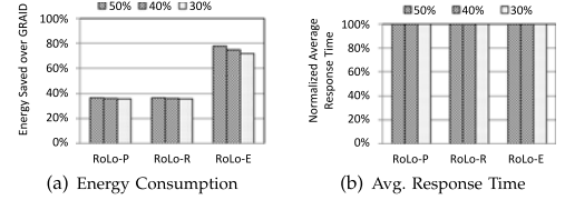
Fig. 9. Energy saved over GRAID and average response time as a function of the amount of free storage space under src2.2 .
