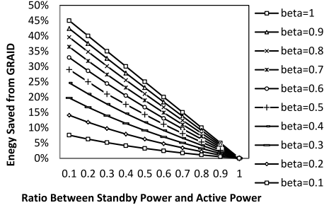
Fig. 6. The Relationship between the Energy of RoLo saved over GRAID and \gamma and \beta .
