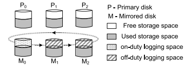
Fig. 2. The basic model of RoLo.
