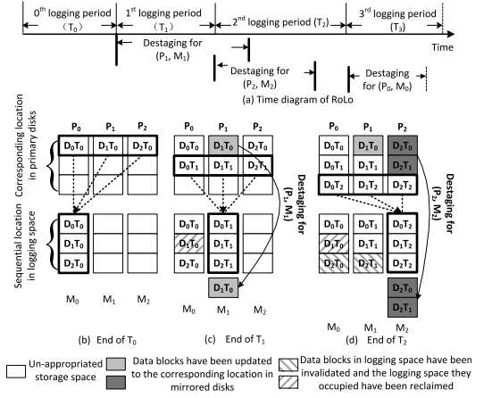
Fig. 4. The decentralized destaging process of RoLo.
