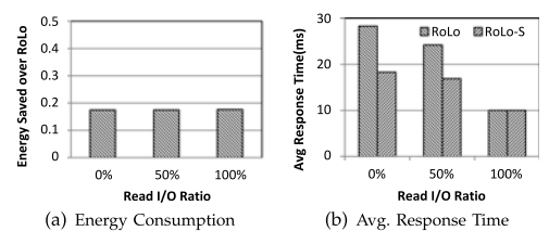
Fig. 13. Energy consumption and performance comparison between RoLo and RoLo-S as a function of read I/O ratio driven by IOMeter.
