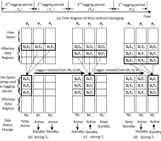
Fig. 3. The dynamic process of logger rotation without destaging. P_i presents the i th primary disk, and M_i represents the P_i 's mirrored disk. The D_m T_n represents the newly written data for the m th mirrored disk pair (P_m, M_m) during the n th logging period T_n .
