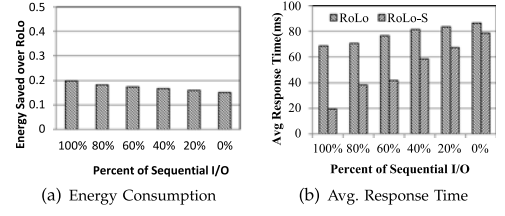
Fig. 12. Energy consumption and performance comparison between RoLo and RoLo-S as a function of sequential I/O ratio driven by IOMeter.
