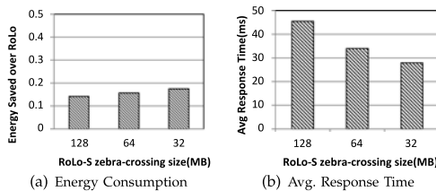
Fig. 11. Energy consumption and performance comparison between RoLo and RoLo-S as a function of zebra-crossing size under src2.2 .
