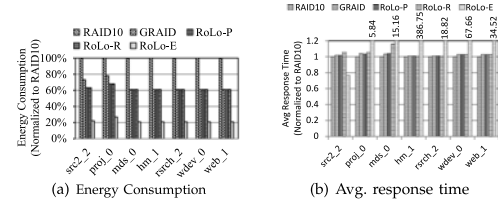
Fig. 8. Energy consumption and average response time, normalized to RAID10, under different traces.
