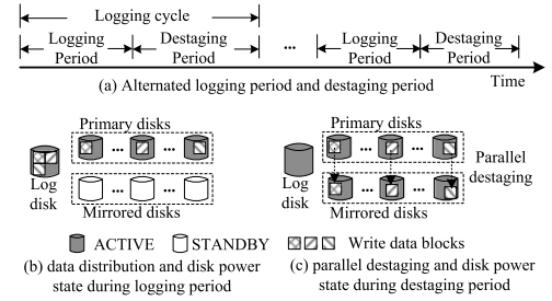
Fig. 1. Working principles of centralized logging and destaging in RAID10 storage architecture.
