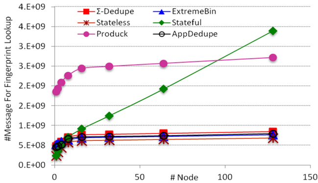
Fig. 11. Communication overhead in terms of the number of fingerprint-lookup message for all seven workloads.
