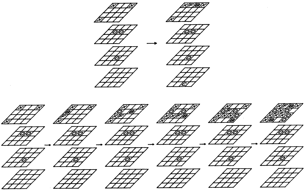
Complications arise in some forced sequences. In the top sequence, if Player X tries to win as in FIGURE 10, Player O's first block at B produces three-in-a-row, forcing Player X to block at C, ending the potential forced sequence. Player X can avoid this by reordering moves as in the bottom sequence.
