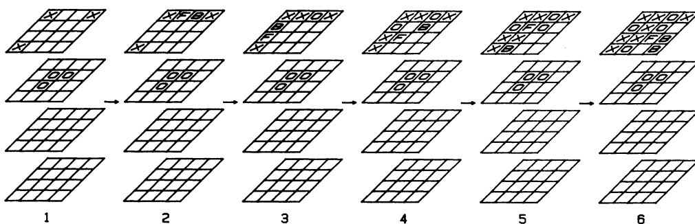
A typical Qubic forced sequence. Player X’s moves at F from each position continually force Player O to block at B , until Player O must block two threes-in-a-row in position 6; since this is impossible, Player O loses.
